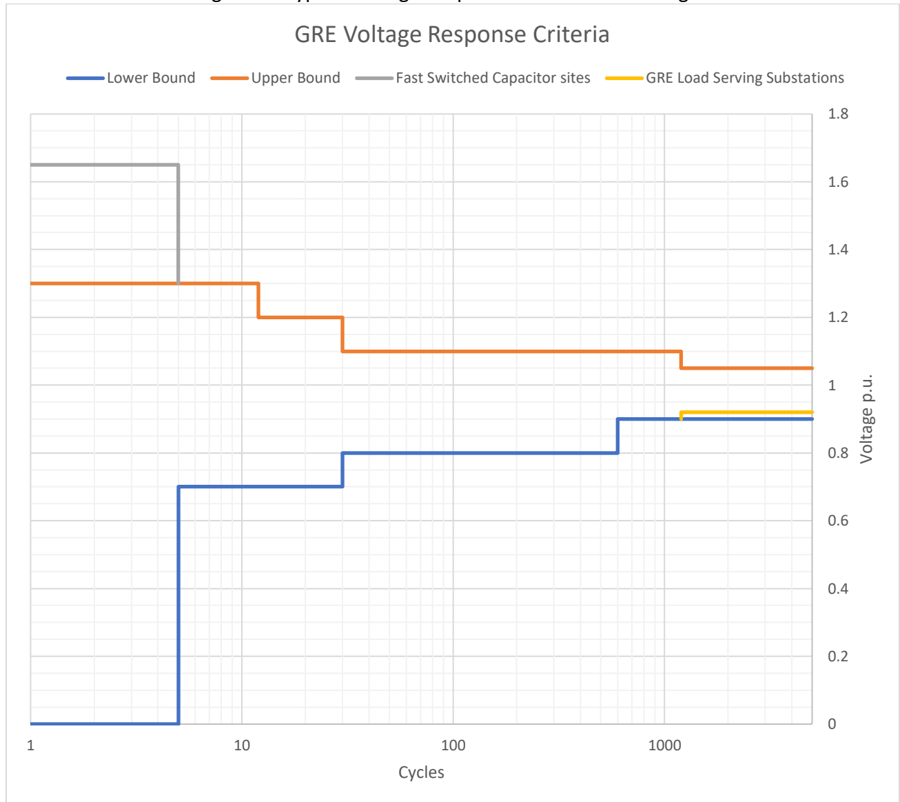
Figure 1: Typical Voltage Response Criteria with timing 11
