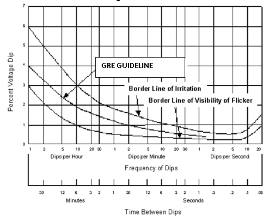
Figure 1 GRE Voltage Flicker Guideline
